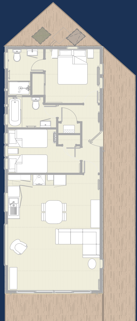
This drawing illustrates the standard floor plan of a 45ft x 16ft floating home (720sq/ft internal space)
